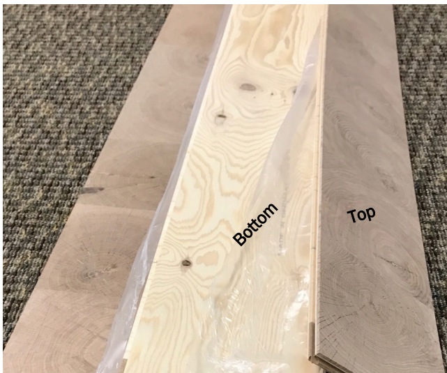
Engineered End Grain planks remain in packaging until installed
